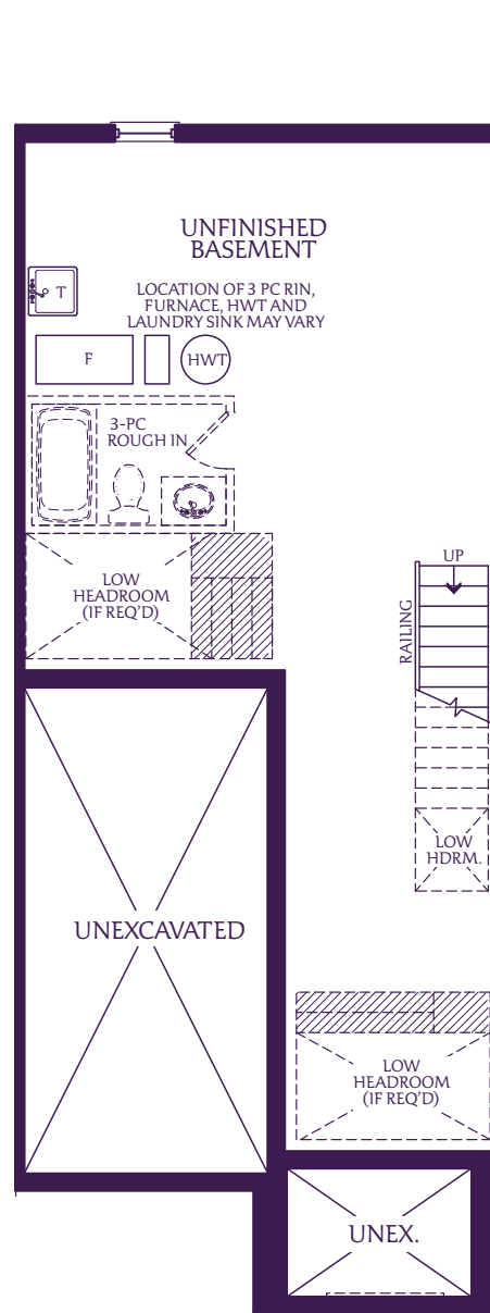
BASEMENT ELEVATION A, B, C & D
