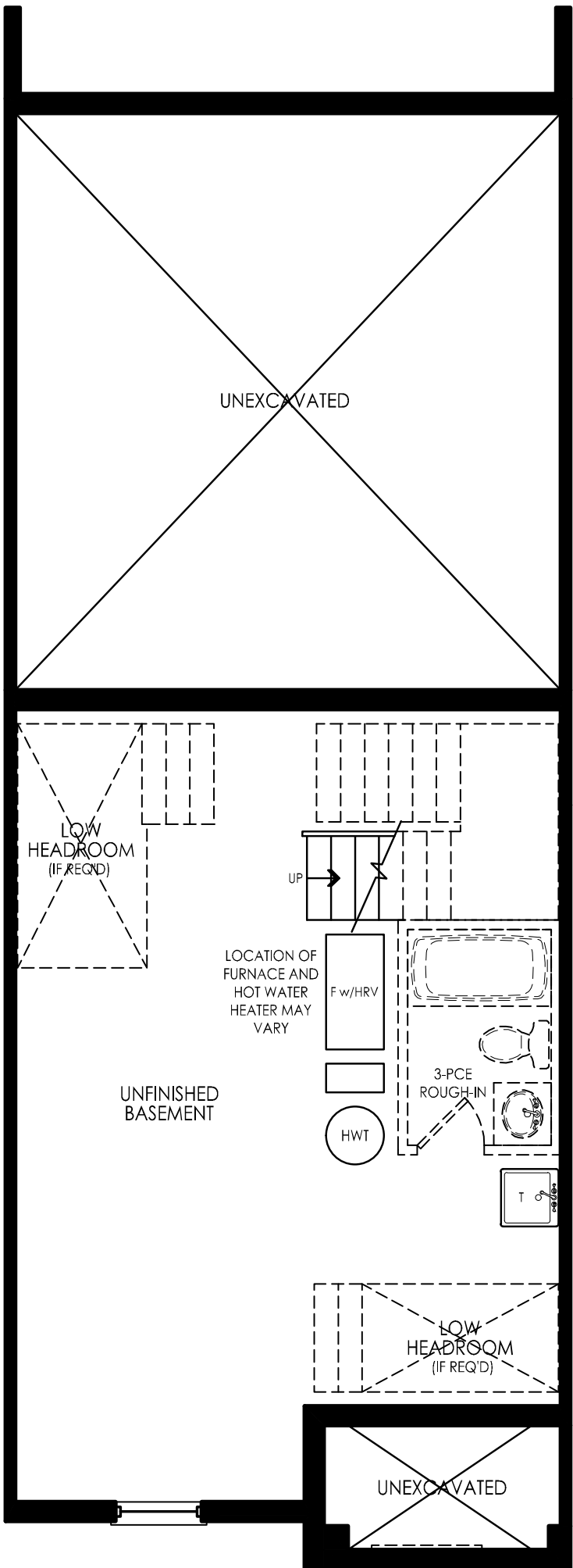
BASEMENT FLOOR ELEV 'A'
